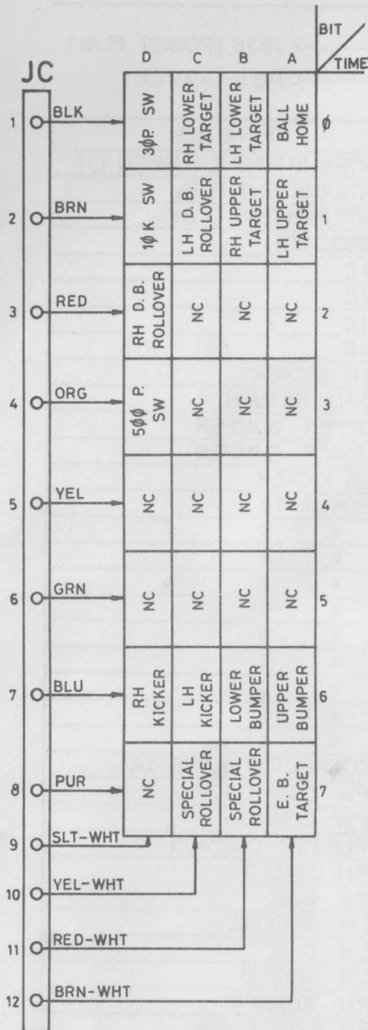
COLOURS (A-B-C-D) WIRED WITH GUIDE
